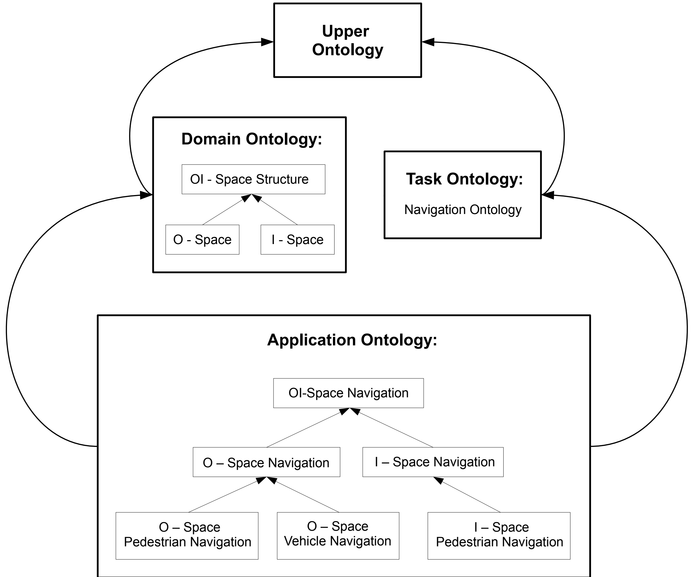
Ontology levels (after Guarino, 1998).
